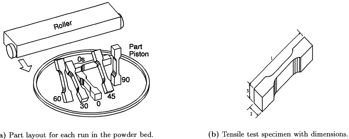
Figure 2: Specimens used in the design of experiments.
