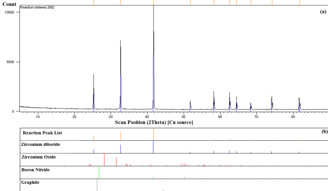
Figure 3: XRD Micrograph of predominant phase of reaction sintered ZrB_2 .
