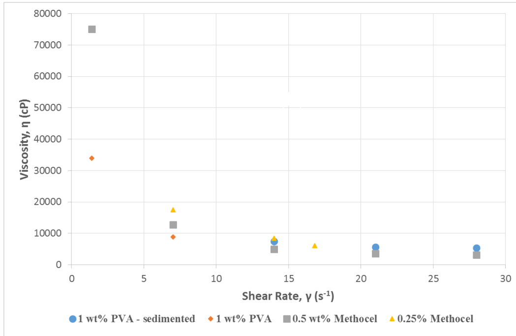
Figure 1: Comparison of PVA and Methocel binders in high solids loading batches.
