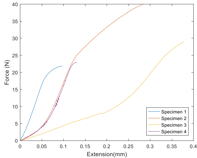
Figure 5 Tensile test for welding copper wire
