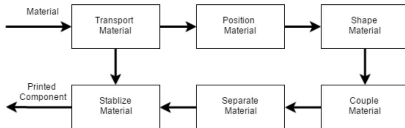
Figure 3. Function structure of additive manufacturing processes
