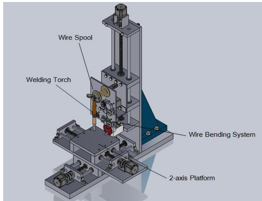
Figure 8. Proposed structure for the metal wire-feed prototyping machine [14]
