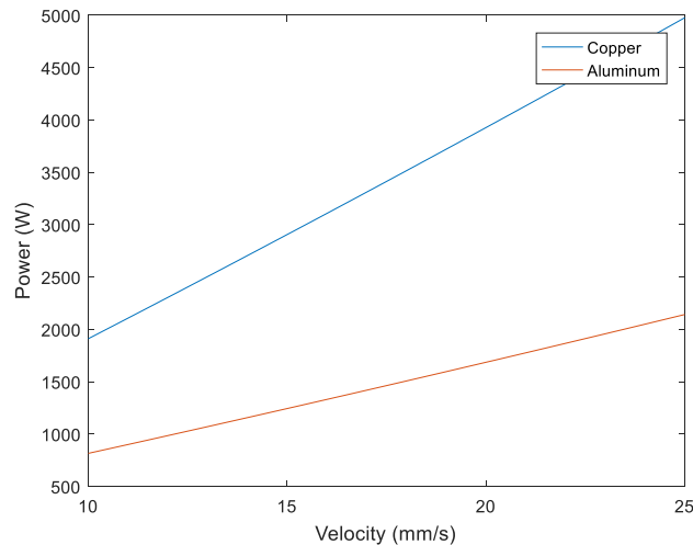
Figure 5. Minimum induction welding power for various velocities
