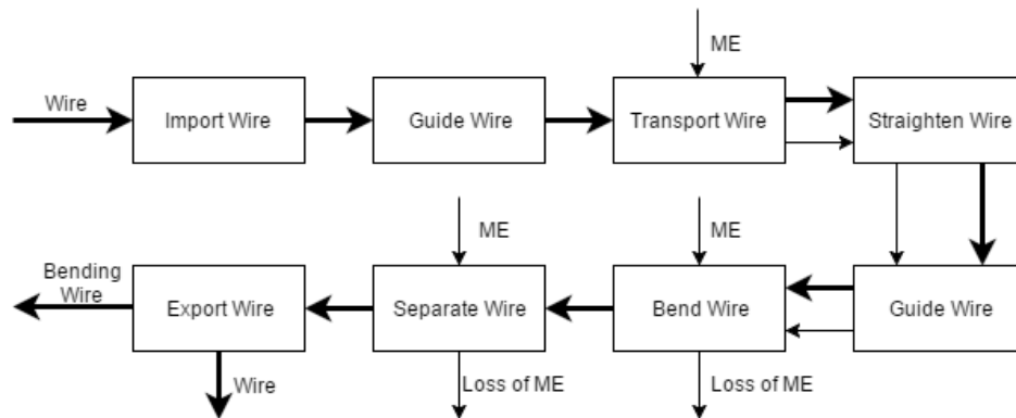
Figure 7. Function structure for a wire bender [14]
