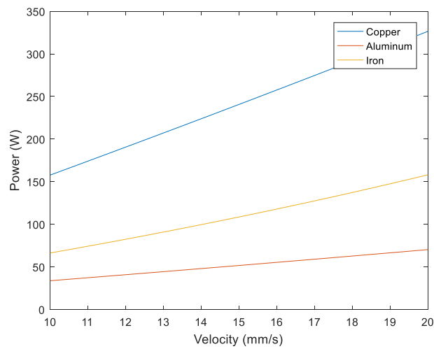
Figure 3. Power requirement for aluminum, copper, and iron for various scanning speeds under CO 2 laser
