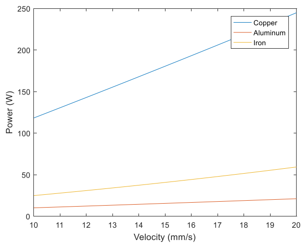
Figure 4. Power requirement for aluminum, copper, and iron for various scanning speeds under Nd:YAG laser
