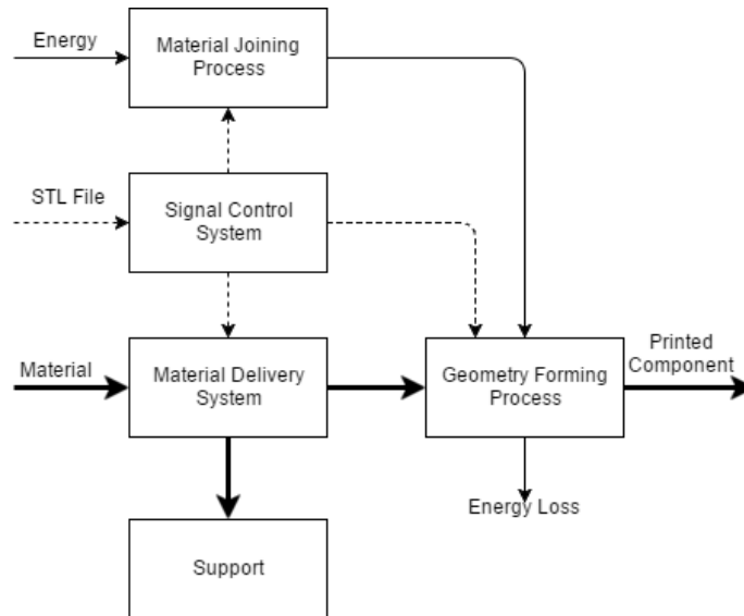
Figure 2. Framework of the additive manufacturing processes
